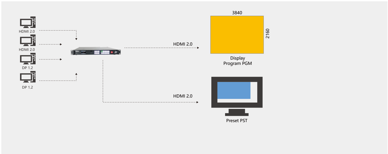
Example: One HDMI source on PGM output with a second HDMI source scaled and configured via output as PST
